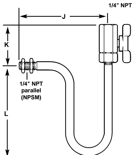
High Pressure
