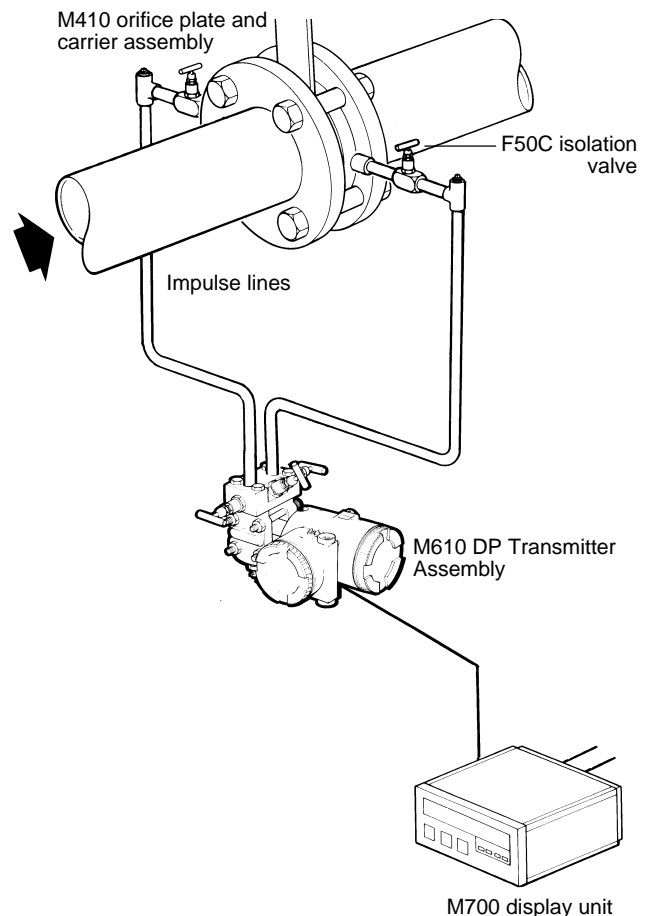
Typical configuration for a non density compensated steam application. Gas applications will differ slightly
